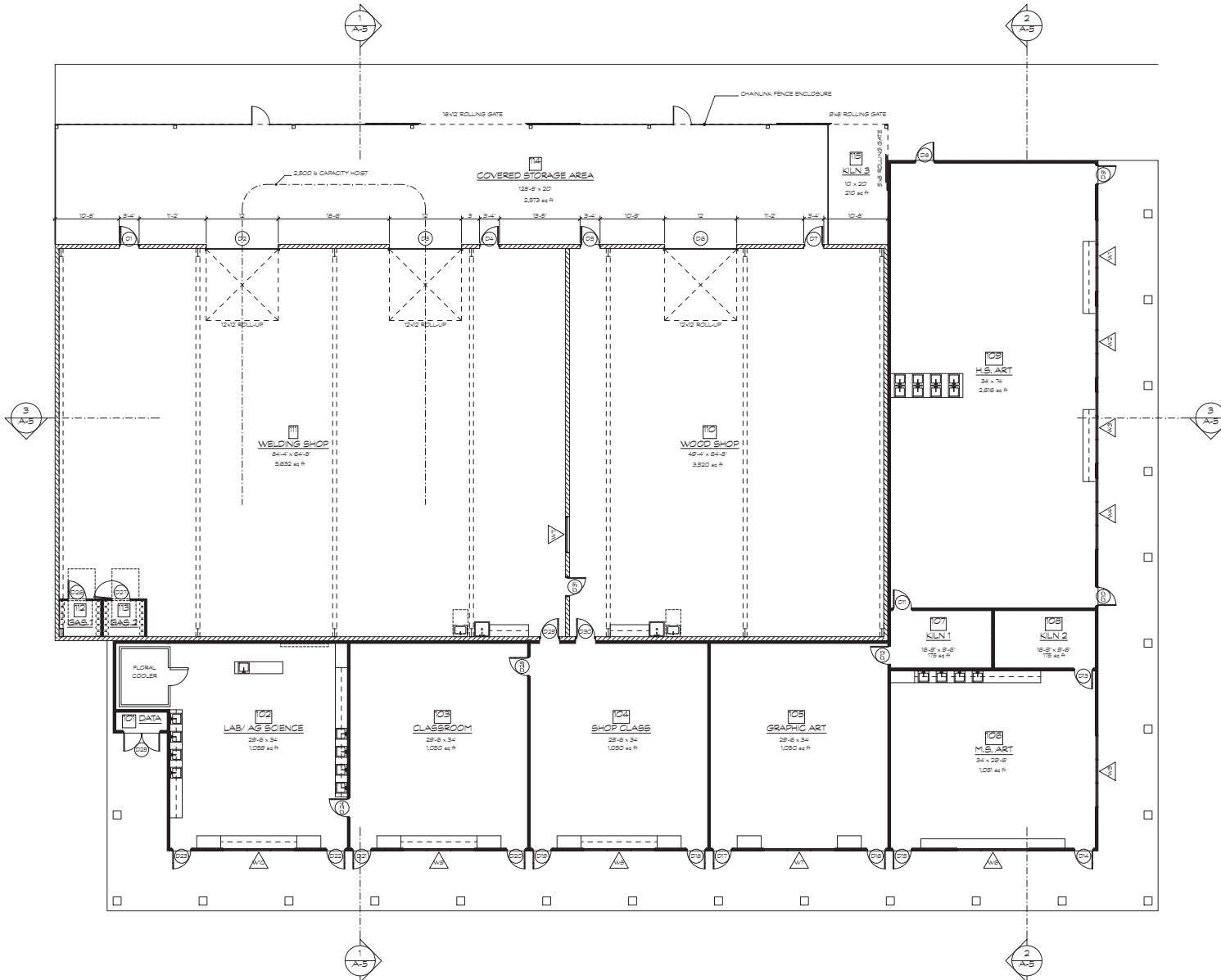
FLOOR PLAN SCALE: 1/8" = 1'-0" 1159 sq ft
